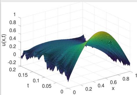
The numerical solution of the stochastic heat equation with boundary conditions that vary stochastically around zero. Notice that despite the stochastic forcing at the boundary we see that dissipation wins. (taken from Lukas Krines' thesis)
